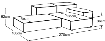
2x element 90x135 + 2x back 90 + arm part 90
