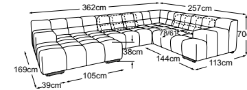
REC left + element 105 without armrest + corner + element arm- rest right incl. 2 MBA Item number: D021130
