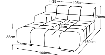
REC armrest left Item number: D021121
