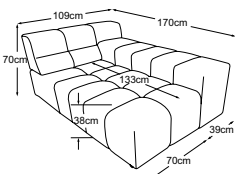
Longchair armrest right
