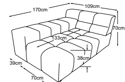
Longchair armrest left
