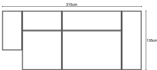
Armrest 90 + element 90x90 + element 90x135 + armrest 135 + back 90 + back 135 (version 1) Item number: D107907
