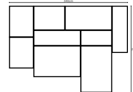
3x element 70x90 + element 70x135 + 2x element 90x135 + armrest 135 + back 90 + back 135 Item number: D107905
