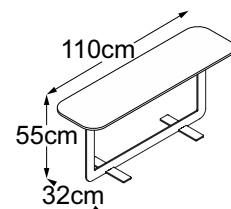
One Blade (Table top: Vetro Marrone) Item number: D1L5VM8
