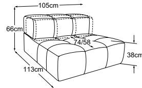
Element 105 without armrest incl. MBA Item number: D088117
