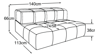
Element 140 without armrest incl. 2 MBA Item number: D088134
