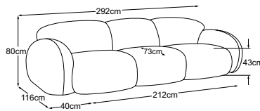
Element 70 AT links + Element 70 + Element 70 AT rechts Bestell-Nummer: D074945
