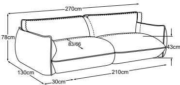
Element 105 armrest left + element 105 armrest right Item number: D073530
