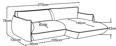
Element 105 armrest left + REC armrest right Item number: D073641
